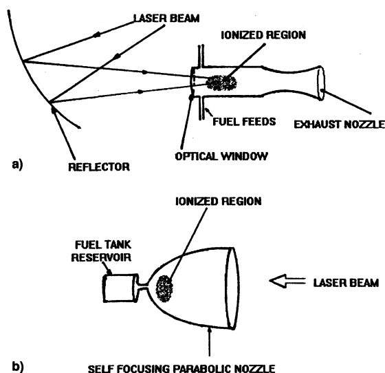
Fig. 1 Laser propulsion system modes of operation: a) continuous wave laser powered and b) repetitively pulsed laser powered.
